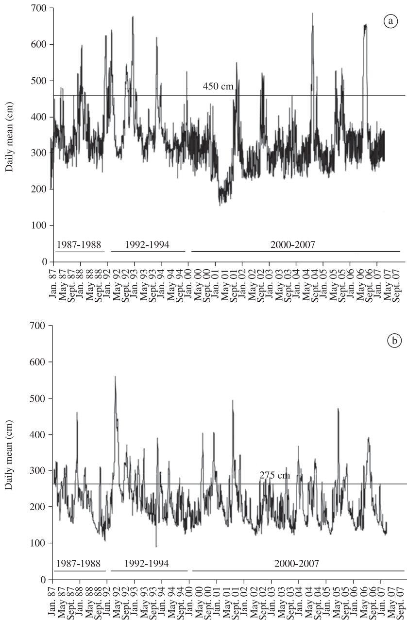
Figure 2. Mean daily water levels of the a) Paraná and b) Ivinheima rivers during the studied period. Dashed lines represent the values from which the rivers overflow onto the adjacent plain.
