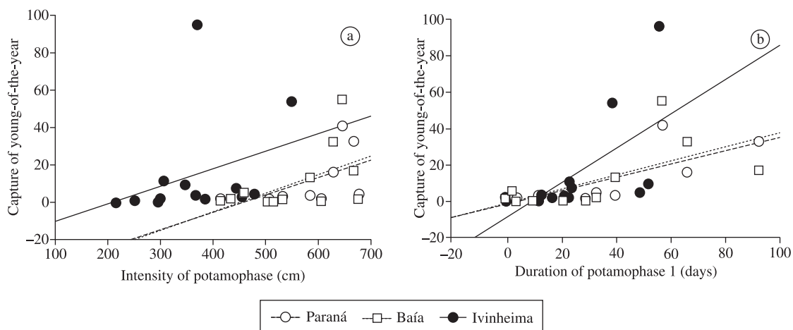
Figure 4. Relationships between abundance of young-of-the-year and hydrographic attributes in the three subsystems.
